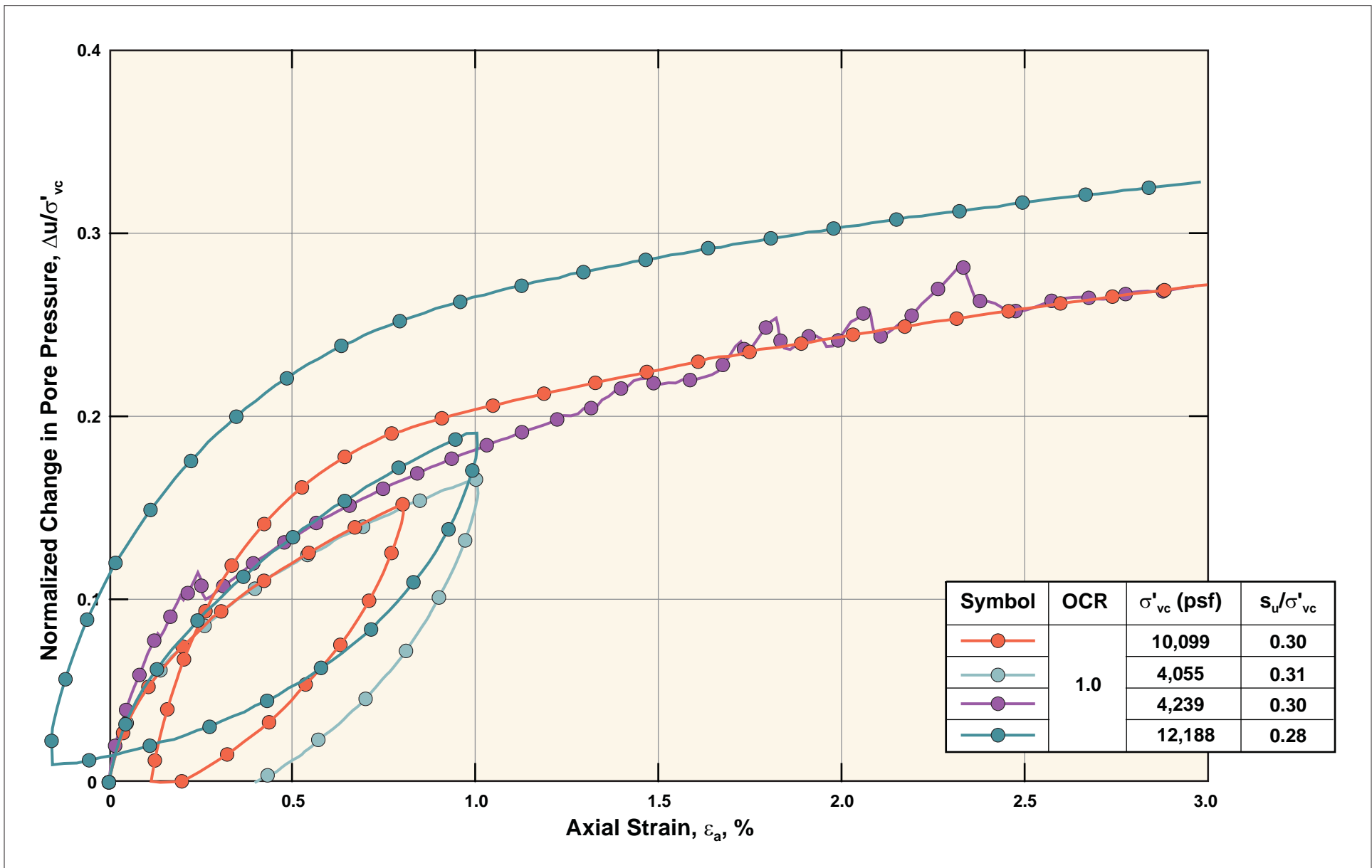
FIG_28: Pore Pressure Behavior from Ko-Triaxial Compression Tests
