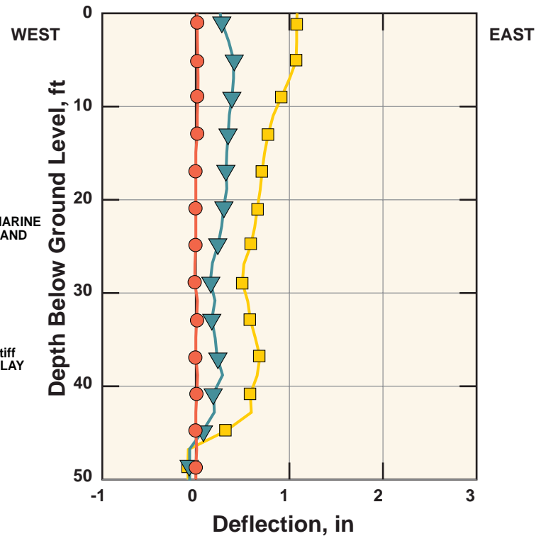
Inclinator I4 Completion of pile driving
