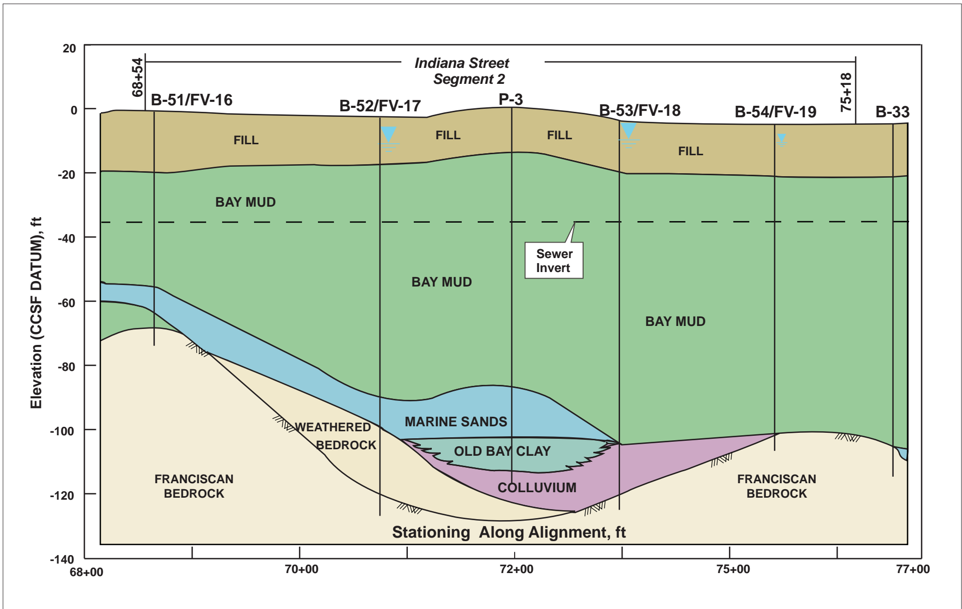
FIG_230 : Subsurface Stratigraphy at Islais Creek Contract D Segment 2: Indiana Street
