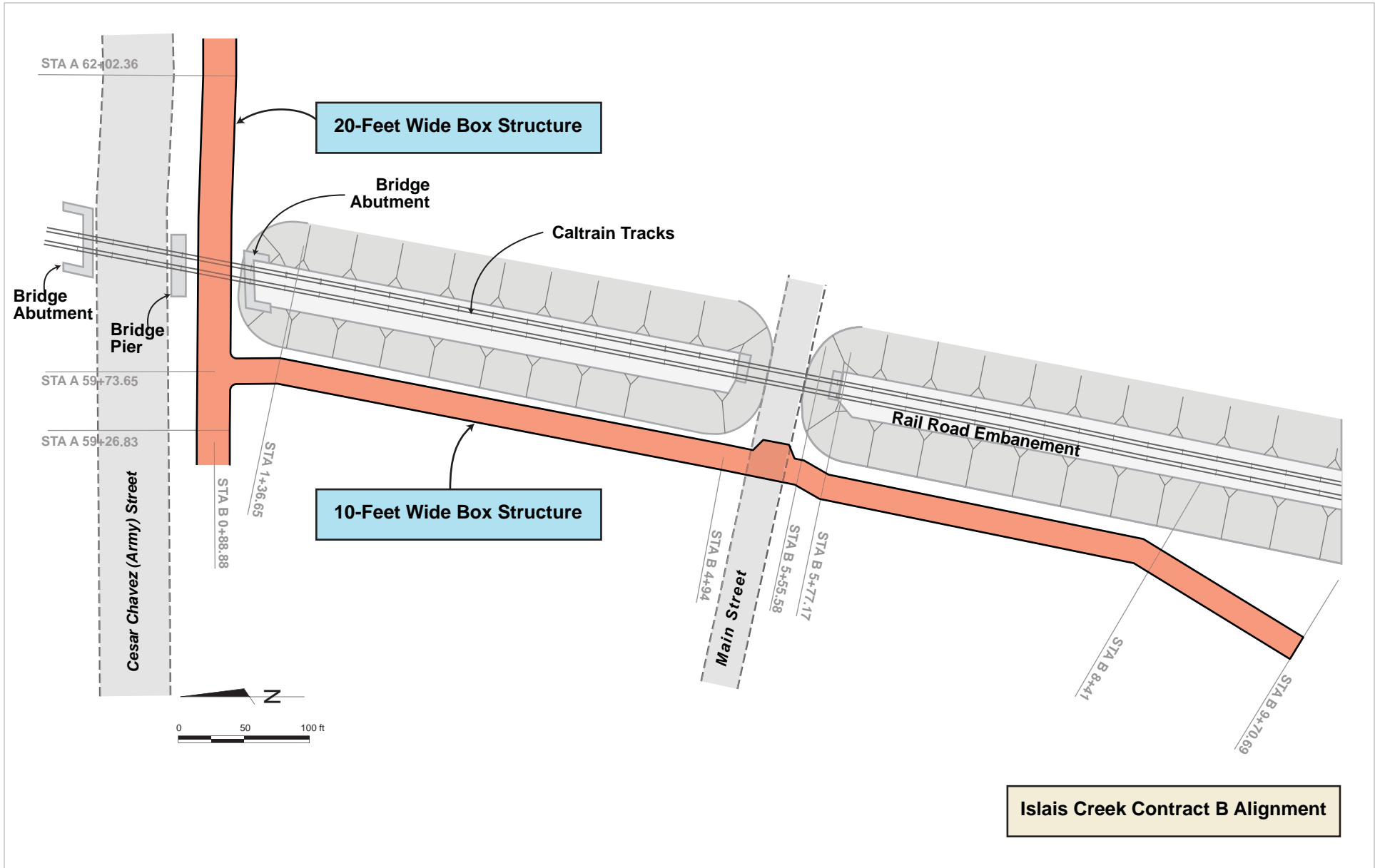
FIG_D-02: Contract B Alignment and Adjacent Structures
