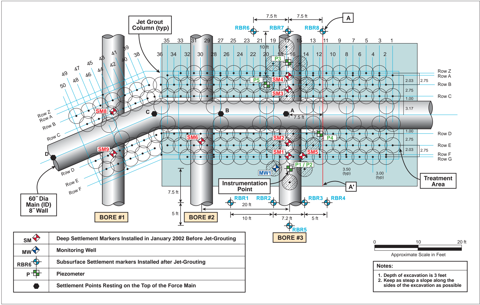
Plate C-15: Excavation Plan
