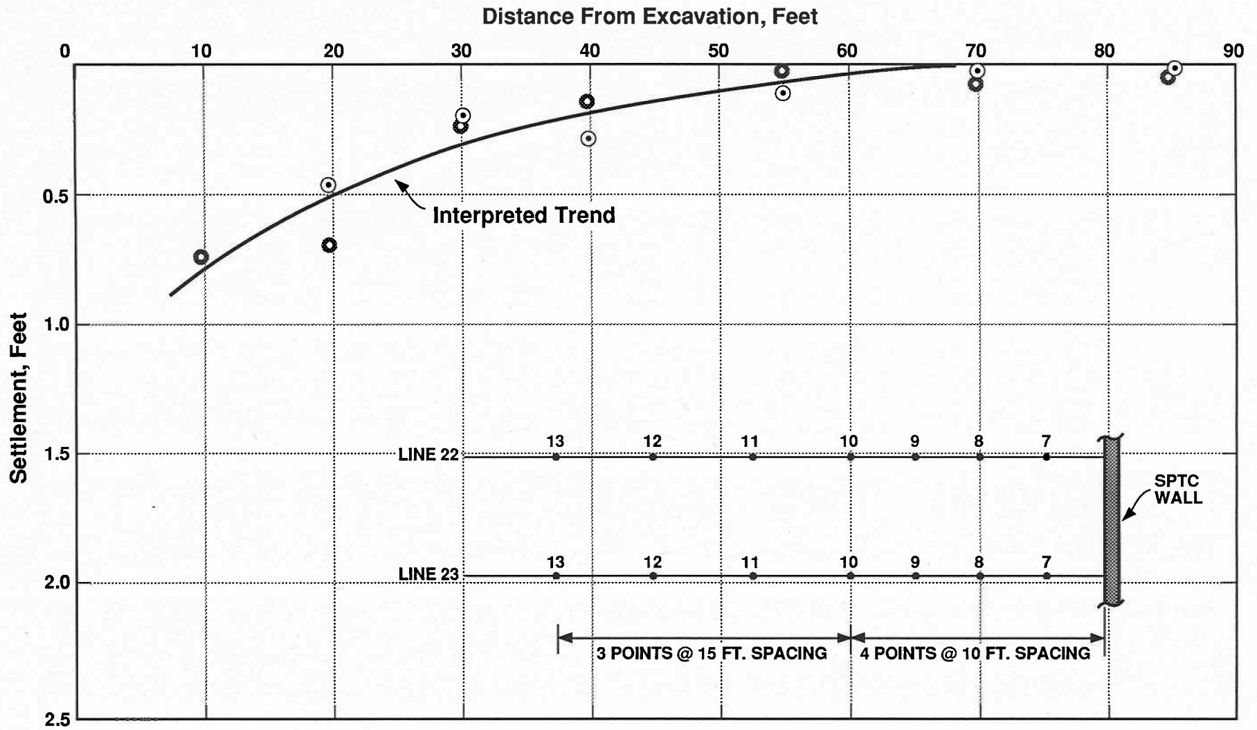
SETTLEMENTS BEFORE EXCAVATION (SUBPAVEMENT SETTLEMENT MARKERS)
