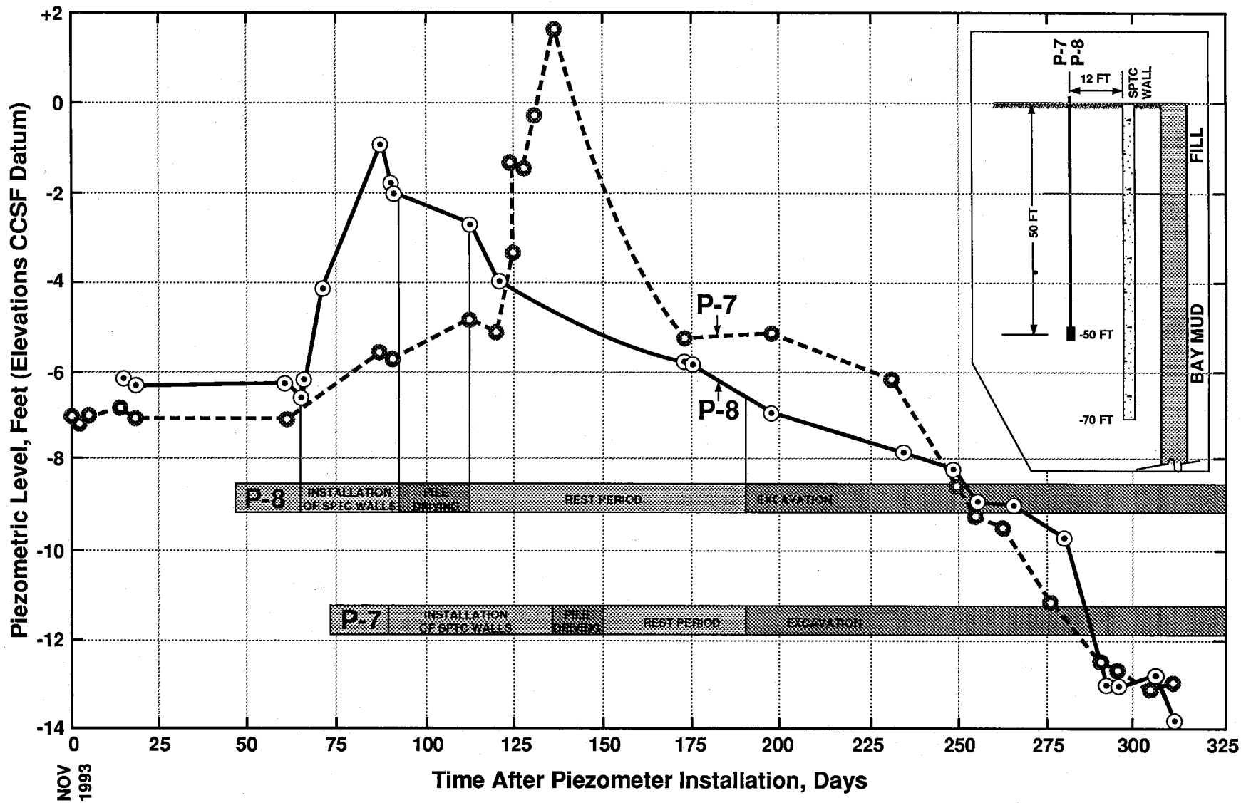
PIEZOMETRIC MEASUREMENTS IN SECTION 1: EFFECTS OF SPTC WALL INSTALLATION, PILE DRIVING AND EXCAVATION
