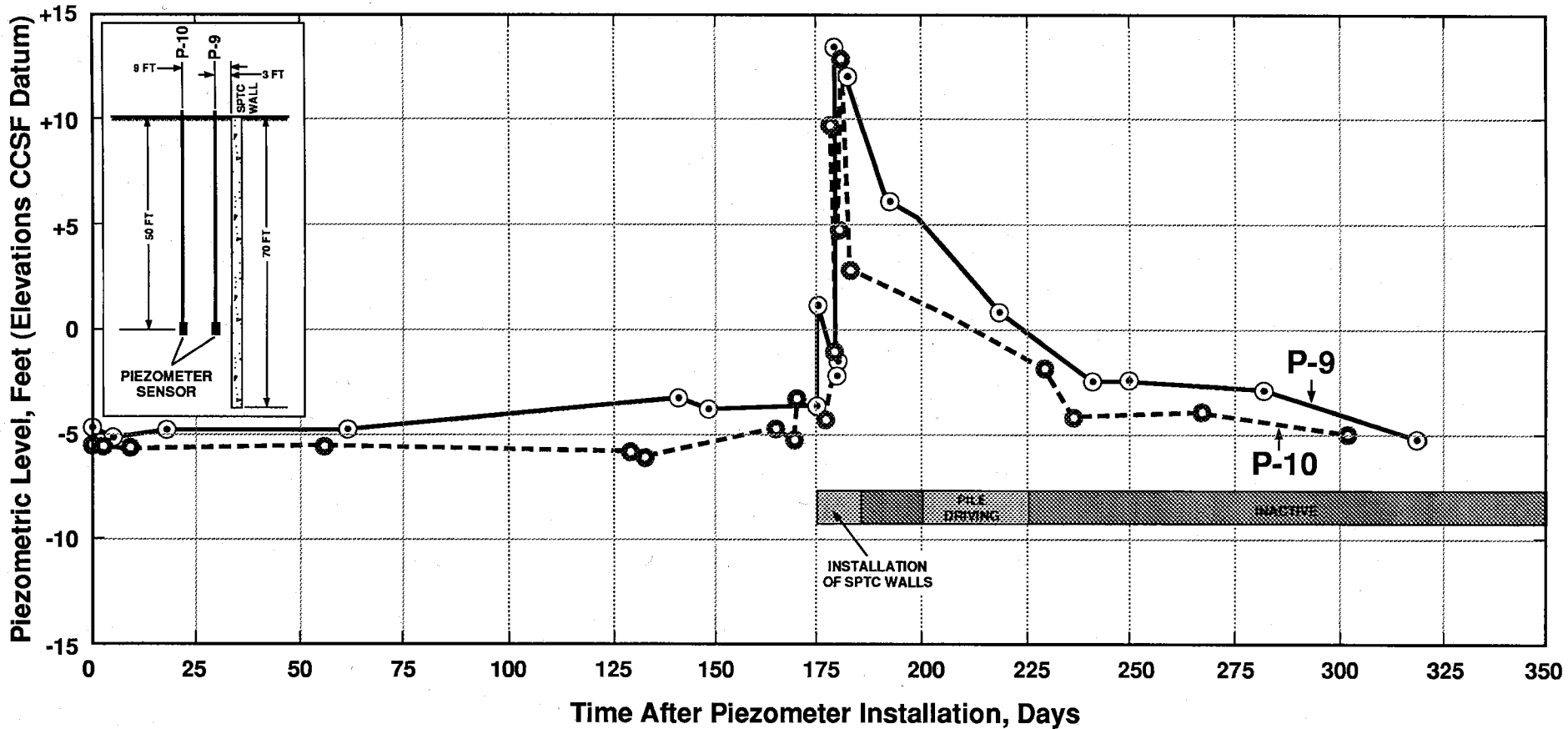
PIEZOMETRIC MEASUREMENTS IN SECTION 2: EFFECTS OF SPTC WALL INSTALLATION AND PILE DRIVING
