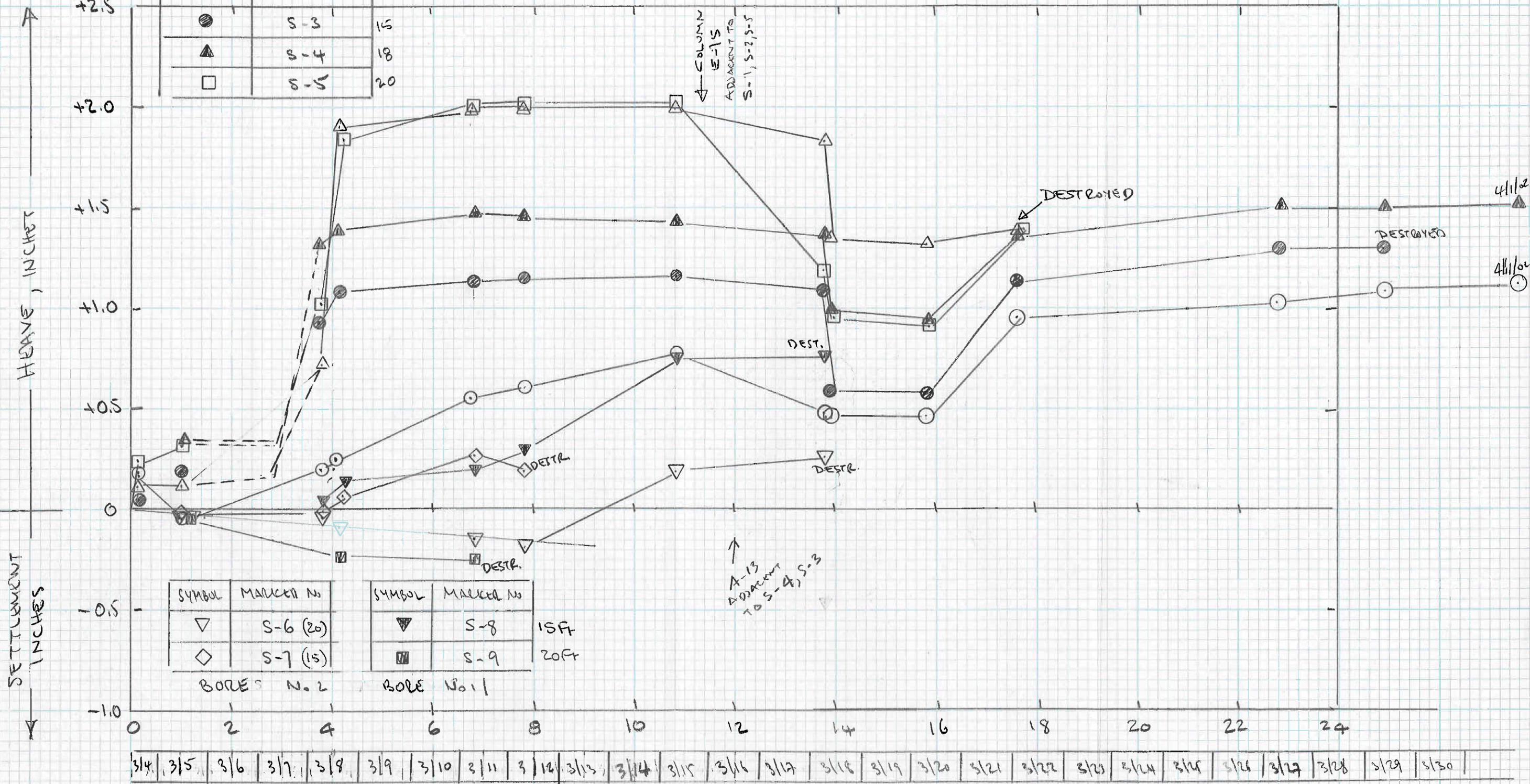
VERTICAL MOVEMENTS OF SETTLEMENT MARKERS VS TIME
