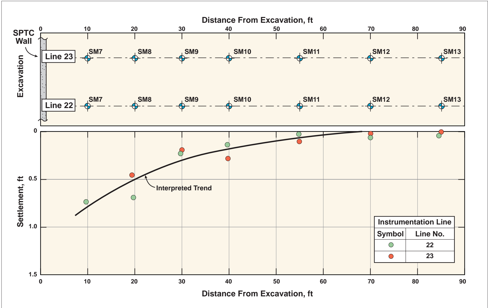
Plate C-08: Settlements Before Excavation (Subpavement Settlement Markers)
