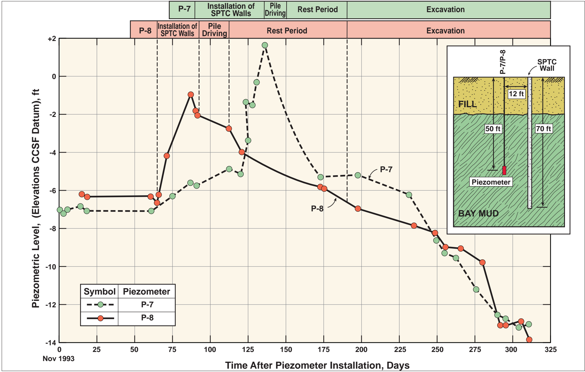
Plate C-09: Piezometric Measurements in Section 1: Effects of SPTC Wall Installation, Pile Driving and Excavation
