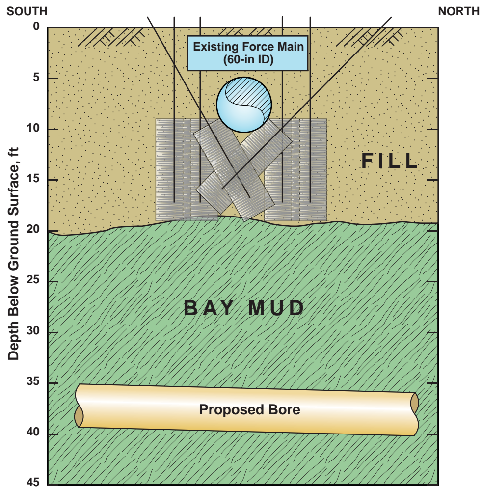
Elevation - Jet Grouting Program
