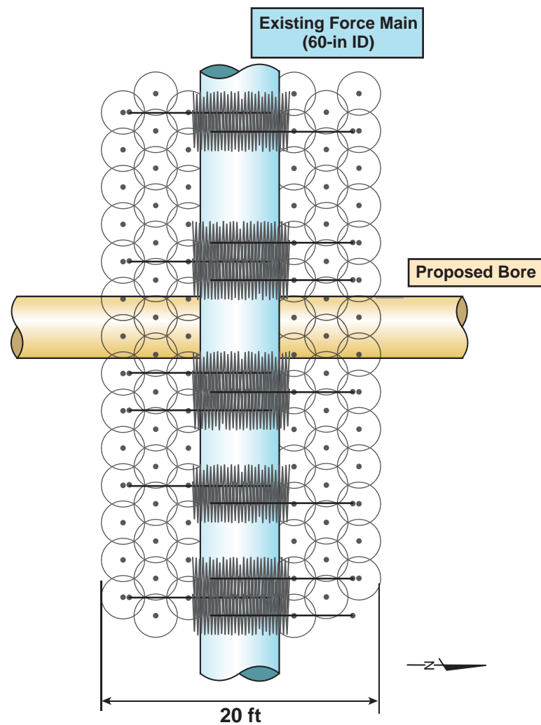
Plan - Proposed Jet Grouting
