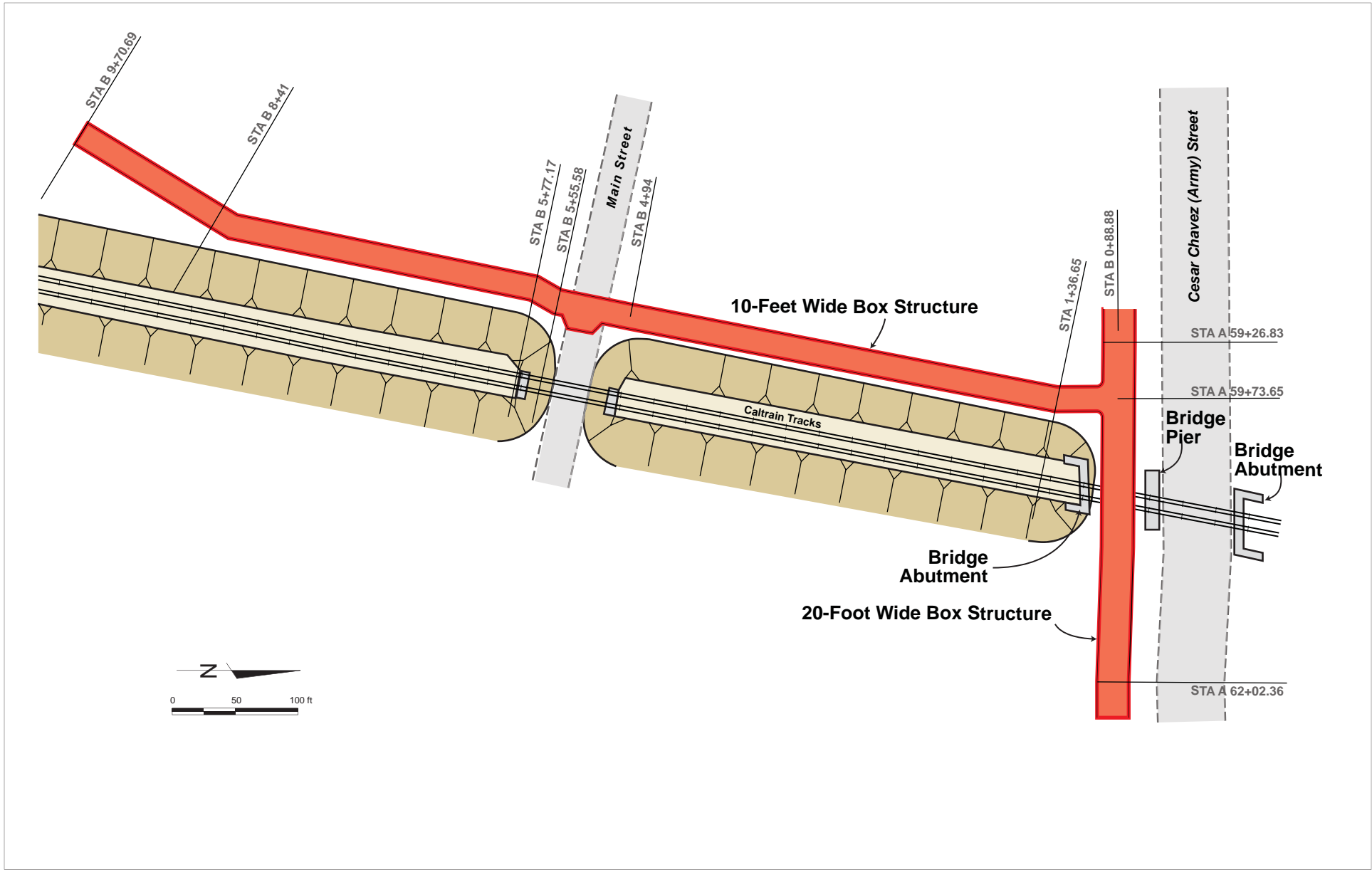
Plate D-02: Contract B Alignment and Adjacent Structures
