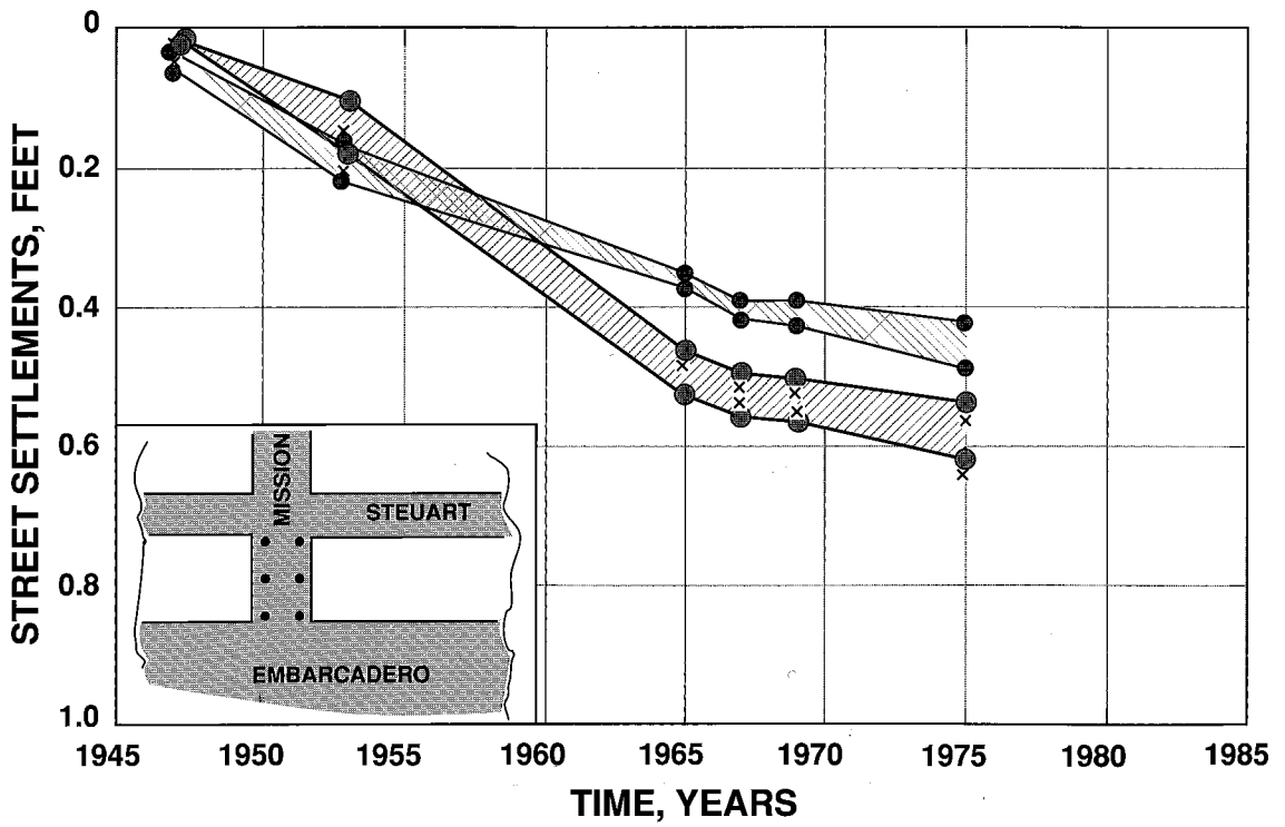
SURFACE SETTLEMENTS MEASURED AT HOWARD AND MISSION STREETS BETWEEN STEUART AND EMBARCADERO
