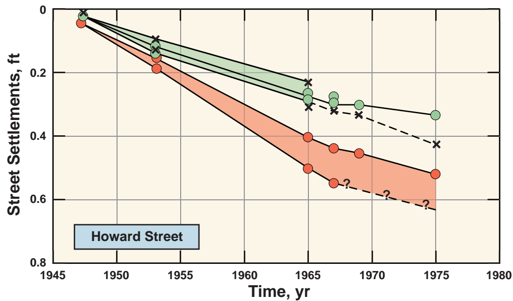
Plate E-05: Surface Settlements Measured at Howard and Mission Streets Between Stuart and Embarcadero
