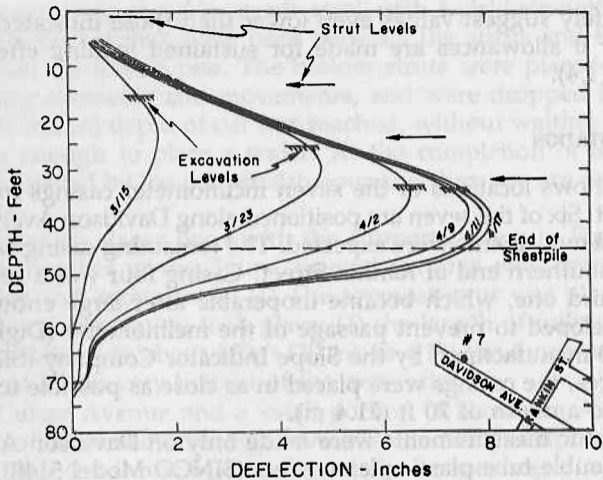
FIG. 9.—Typical Measured Lateral Movements for Deepening Excavation on Davidson Avenue—Inclinometer No. 7 (1 ft = 0.305 m; 1 in. = 25.4 mm)
