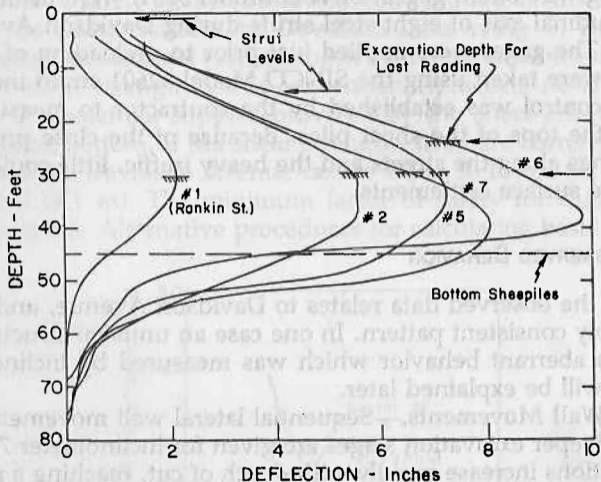
FIG. 10.—Maximum Measured Lateral Movements in All Inclinometers except Nos. 3 and 4 (1 ft = 0.305 m; 1 in. = 25.4 mm)
