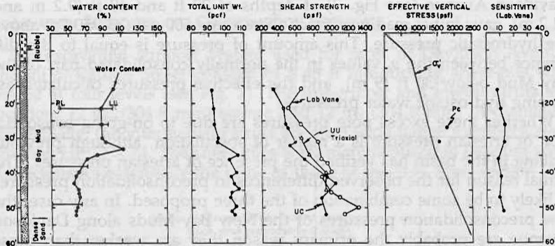
FIG. 5.—Soil Properties—Custer Avenue and Rankin Street (1 psf = 47.9 Pa; 1 pcf = 1.6 kg/m 3 )
