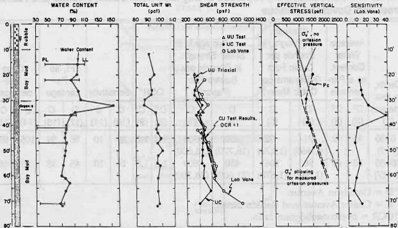
FIG. 6.—Soil Properties—Davidson Avenue (1 psf = 47.9 Pa; 1 pcf = 1.6 kg/m 3 )
