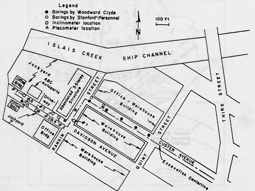
FIG. 3.—Plan View Showing Culvert Alinement and Locations of Borings and Instrumentation (1 ft = 0.305 m)
