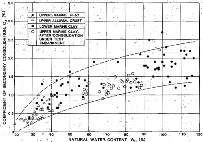
FIG. 9.—Correlation of Coefficient of Secondary Consolidation with Natural Water Contents
