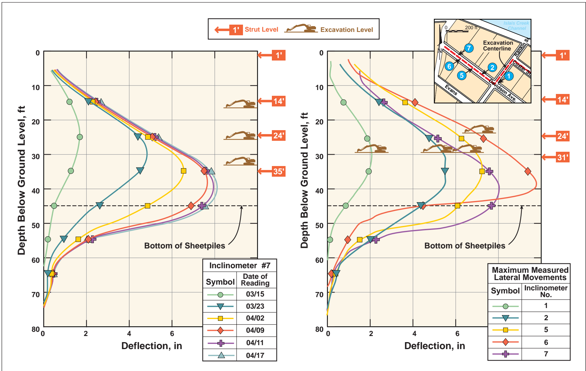
Plate F-01: Figure A: Typical Measured Lateral Movements for Deepening Excavation on Davidson Avenue-Inclinator No. 7 Figure B: Maximum Measured Lateral Movements in All Inclinator Nos. Except Nos. 3 and 4
