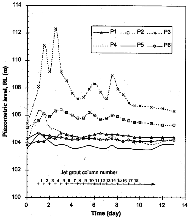
Fig. 9. Changes in piezometric level during jet-grouting trial.
