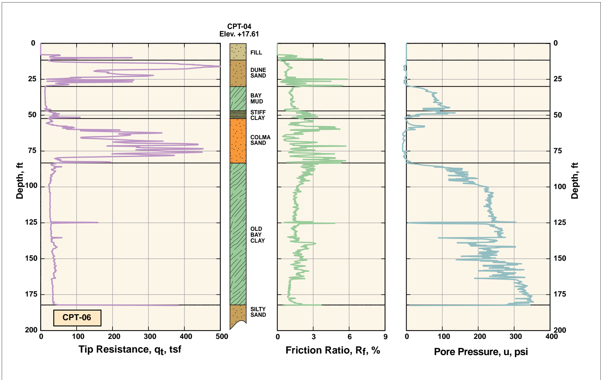
Plate MIS-CPT.06: Results of Cone Penetration Test: CPT-06
