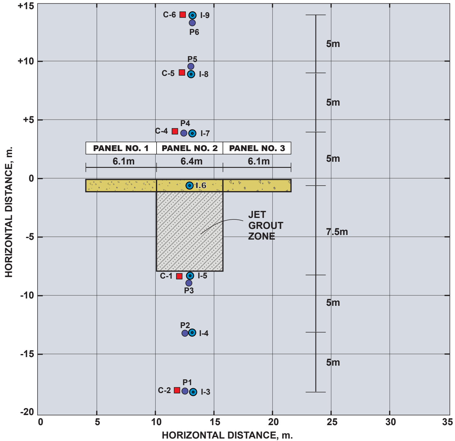
PLAN OF SINGAPORE JET-GROUT EXPERIMENT
