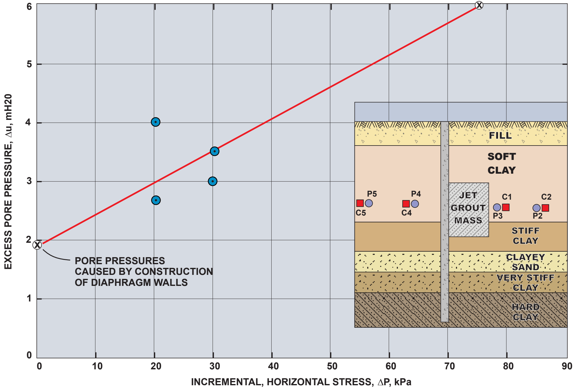
INCREMENTAL PORE PRESSURES VS. INCREMENTAL TOTAL STRESSES MEASURED IN THE SOFT CLAY SINGAPORE EXPERIMENT
