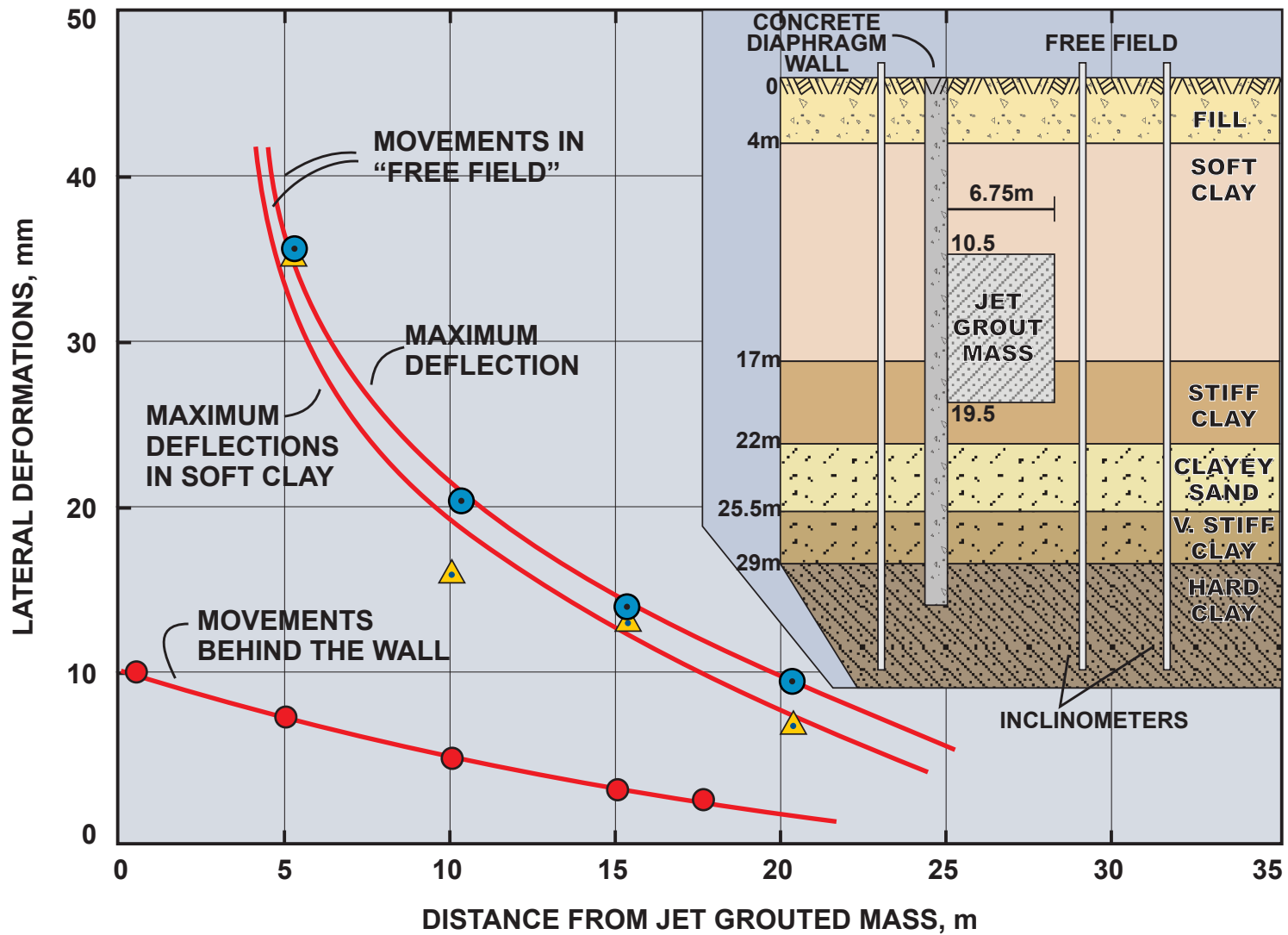
LATERAL DEFLECTIONS CAUSED BY JET-GROUTING SINGAPORE EXPERIMENT
